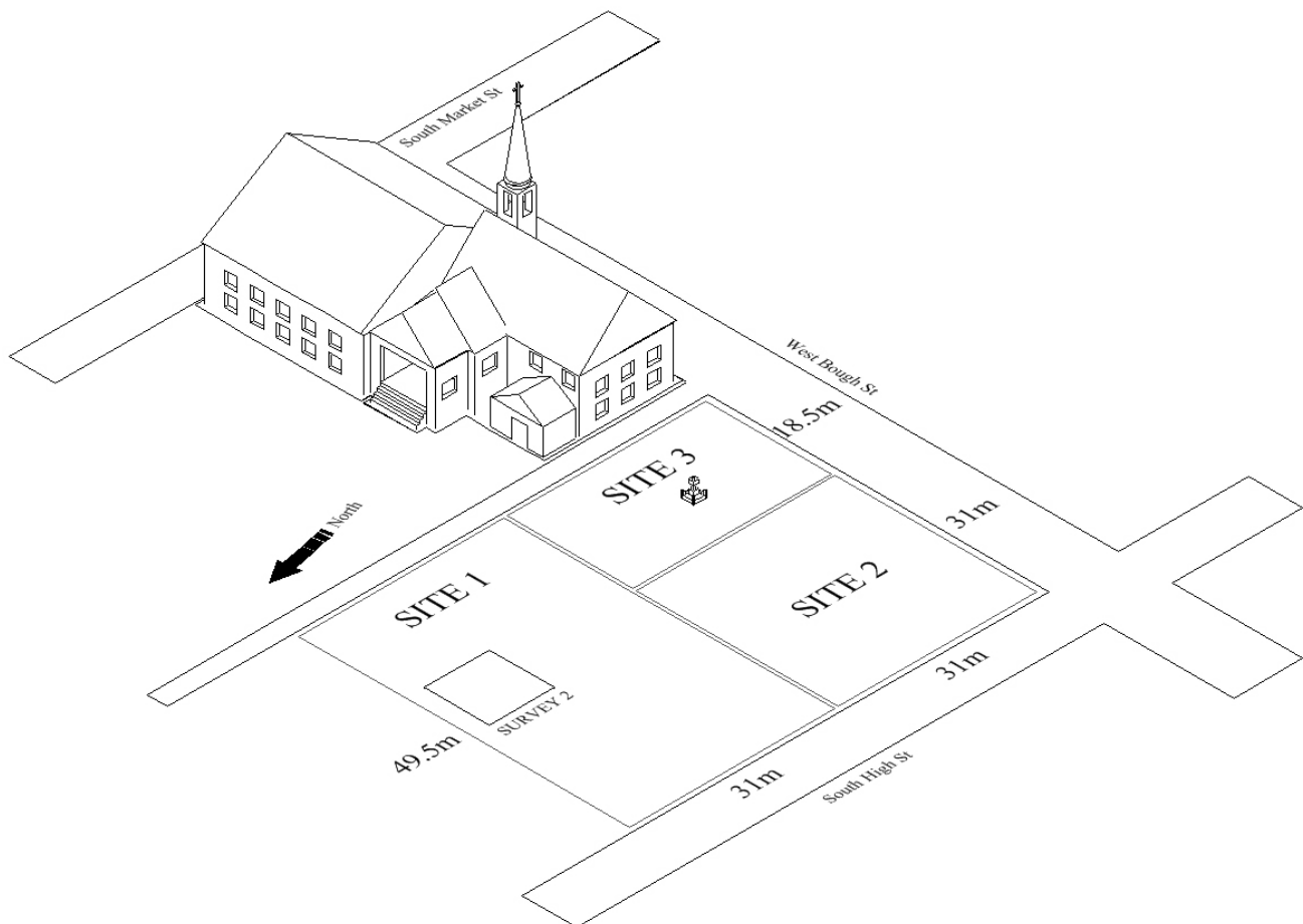
Figure 3: Drawing of Sharon Lutheran Church showing the first GPR Survey with the three sites surveyed taken at 50 cm spacing and the 10x10 m 2 site of the second survey within Site 1.
