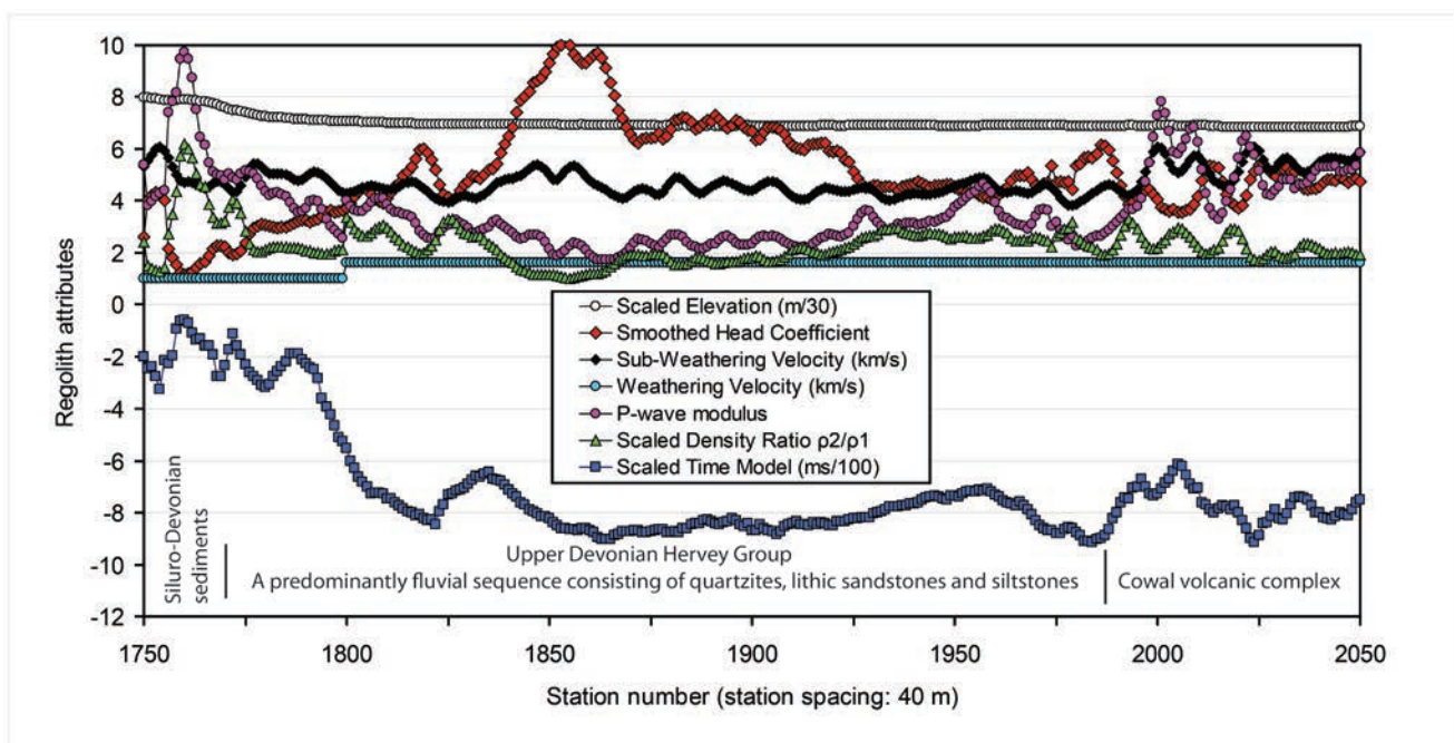
Figure 7: Summary of refraction attributes derived from traveltme and amplitude data.
